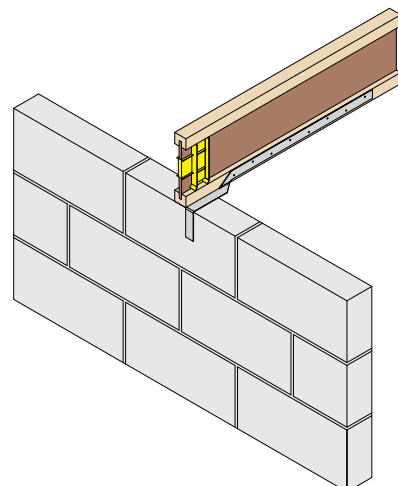
I-Joist End Seal Pages 30 - 31
